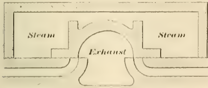
FIG. 1. PLAIN D-VALVE.
